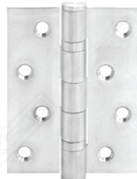
ESS EL 4X3X3MM 2BB SSS Capacity (max) : 75 KG / pair
