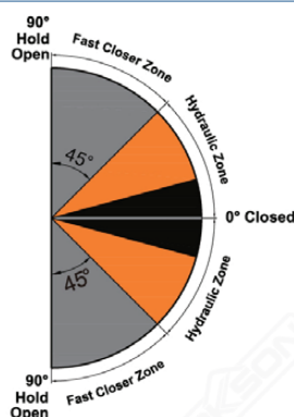
SHH 502 MATT BLACK (GLASS TO WALL)
